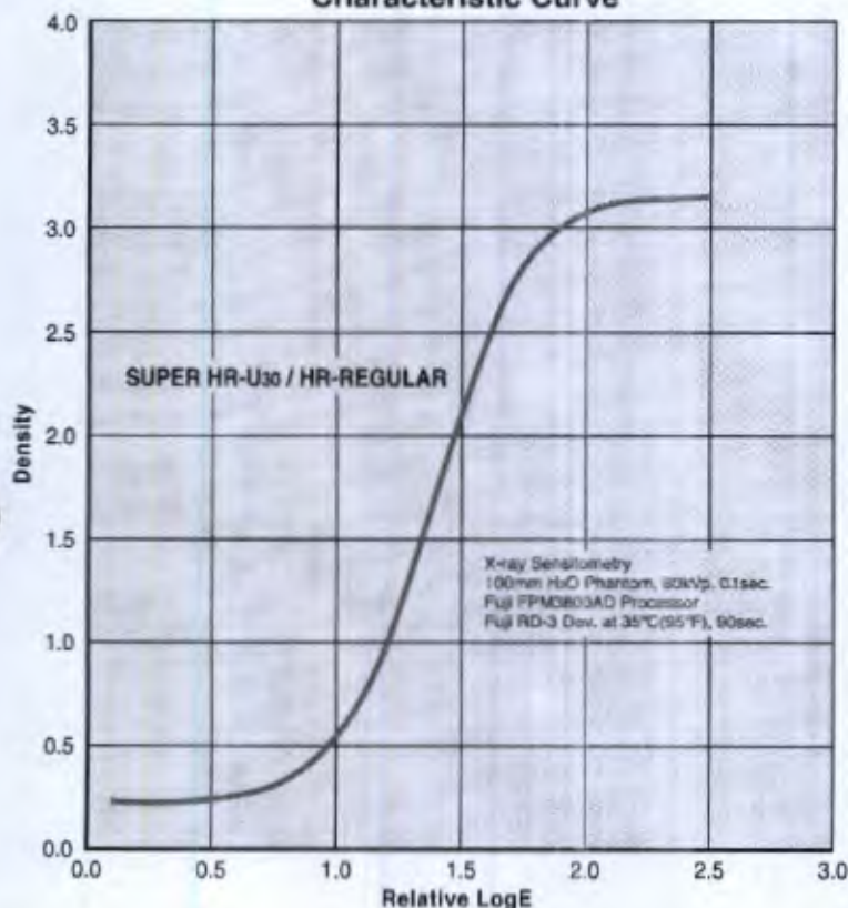
Characteristic Curve
