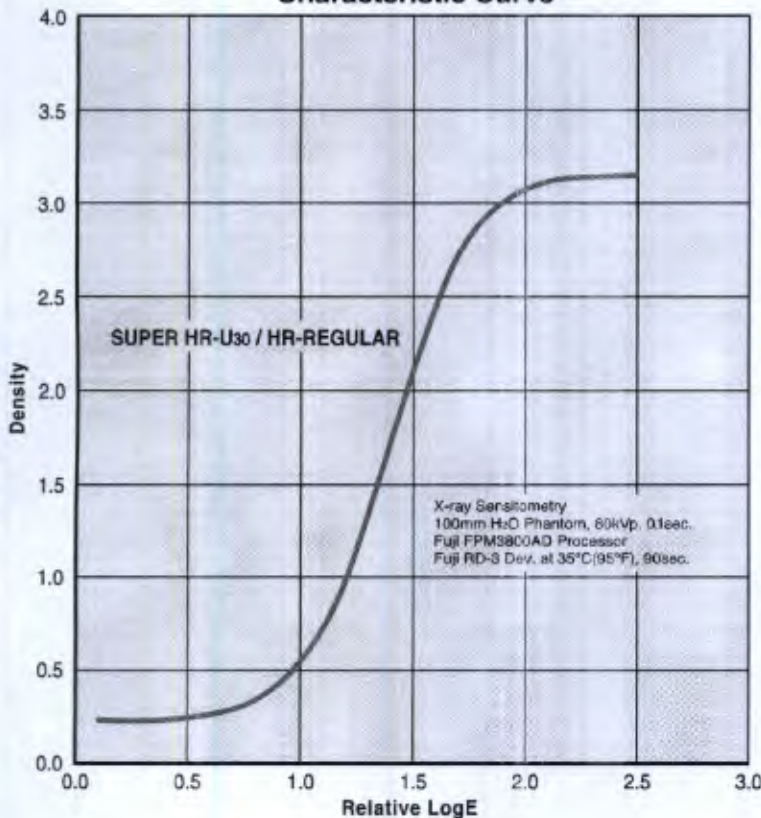
Characteristic Curve
